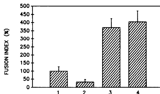
Fig.2. The effect of PEG impurities on PEG-induced cell fusion. Fusion obtained with: (1) commercial PEG; (2) PEG purified according to [10]; (3) 2.5 \times 10^{-5} M SDS, then commercial PEG; (4) 2.5 \times 10^{-5} M SDS, then purified PEG.
